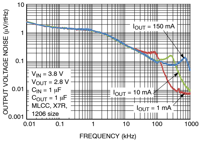
Figure 30. Output Voltage Noise Spectral Density for V_{\text{OUT}} = 2.8 \text{ V} , C_{\text{OUT}} = 1 \mu\text{F}
