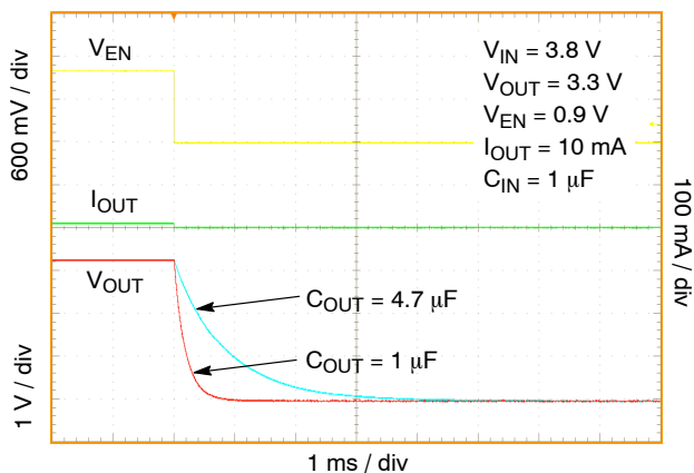
Figure 38. Enable Turn-off Response
