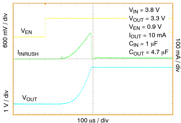
Figure 36. Enable Turn-on Response – C_{OUT} = 4.7 \mu F
