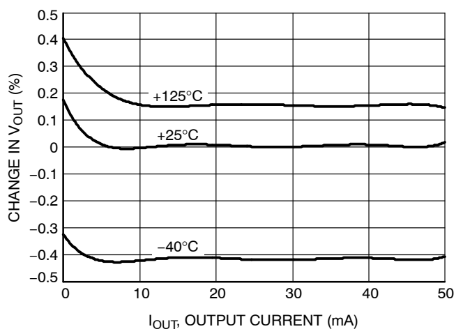
Figure 7. Load Regulation
