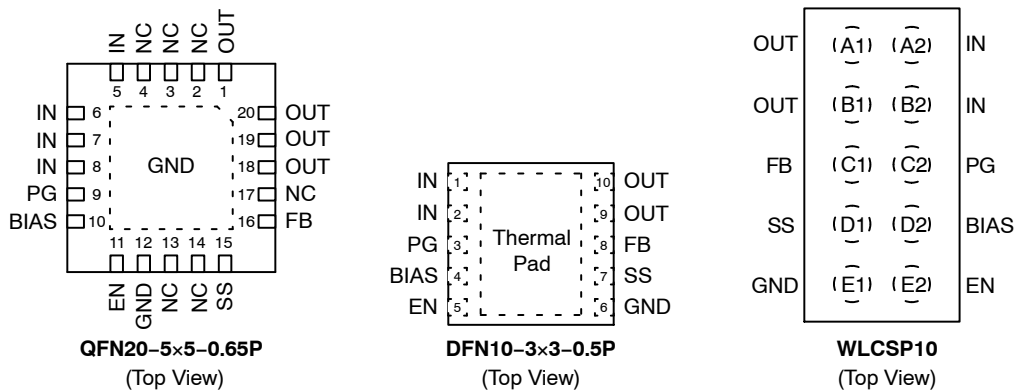
Figure 2. Pin Connections
