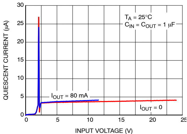
Figure 14. NCV8716x15xxx Ground Current vs. Input Voltage
