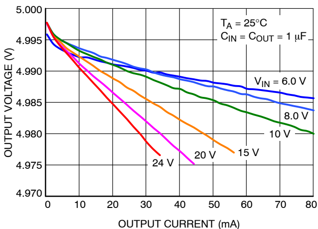
Figure 10. NCV8716x50xxx Output Voltage vs. Output Current
