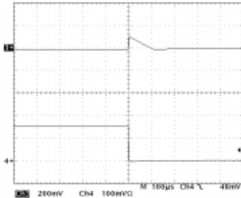
Figure 3. Turn-ON Response
