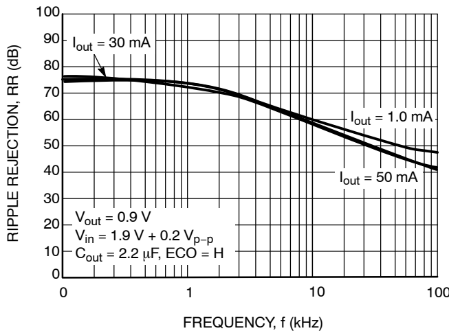
Figure 24. Ripple Rejection vs. Frequency
