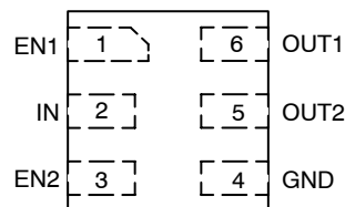
WDFN6 (Top View)
