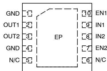
DFN10 (Top View)
