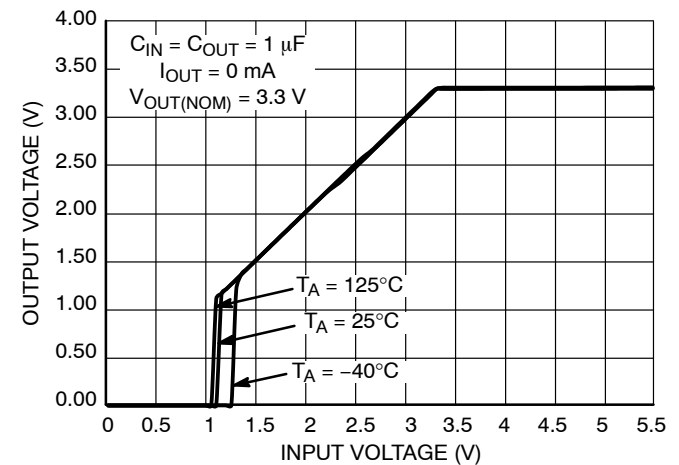
Figure 20. Output Voltage vs. Input Voltage V_{OUT} = 3.3\ \text{V}
