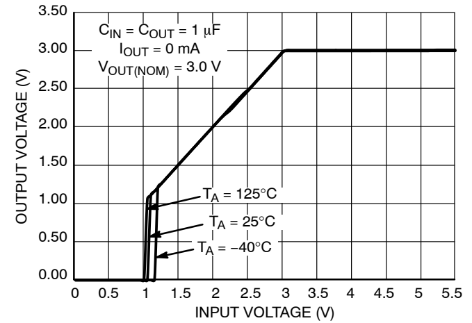
Figure 18. Output Voltage vs. Input Voltage V_{OUT} = 3.0\ \text{V}
