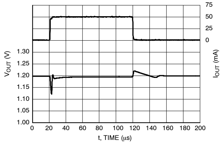
Figure 53. Load Transients, 1.2 V Version, I_{OUT} = 1 - 50 \text{ mA} , t_R = t_F = 0.5 \text{ } \mu\text{s} , V_{IN} = 2.2 \text{ V} , AE = 0 \text{ V}
