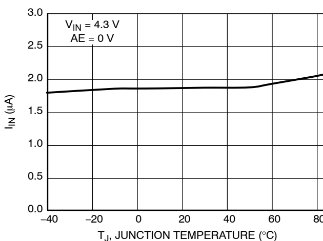
Figure 30. Supply Current vs. Temperature, 3.3 V Version
