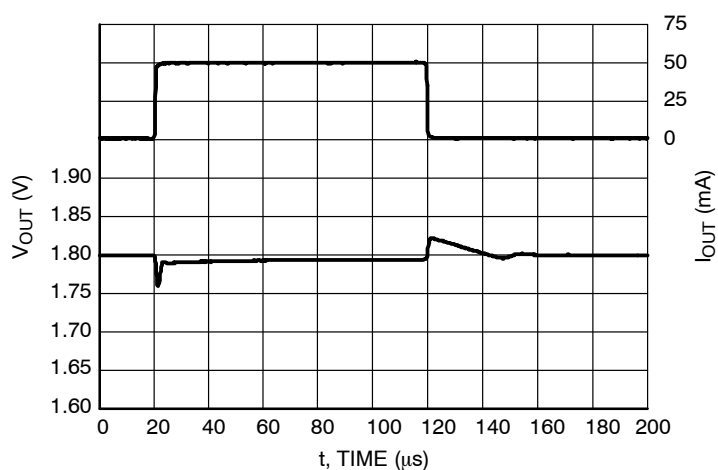
Figure 56. Load Transients, 1.8 V Version, I_{OUT} = 1 - 50 \text{ mA} , t_R = t_F = 0.5 \mu\text{s} , V_{IN} = 2.8 \text{ V} , AE = V_{IN} \text{ V}
