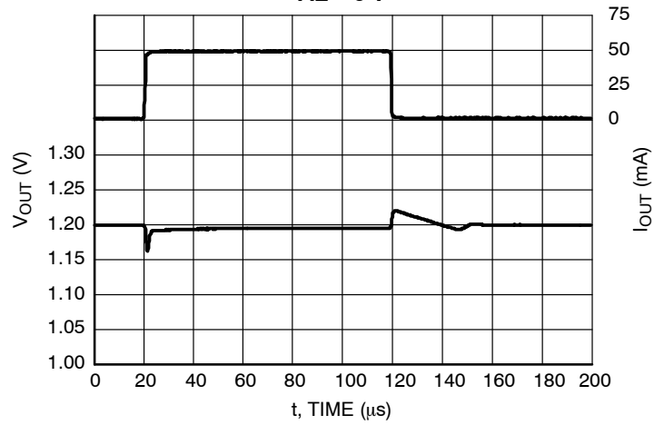
Figure 54. Load Transients, 1.2 V Version, I_{OUT} = 1 - 50 \text{ mA} , t_R = t_F = 0.5 \text{ } \mu\text{s} , V_{IN} = 2.2 \text{ V} , AE = V_{IN} \text{ V}
