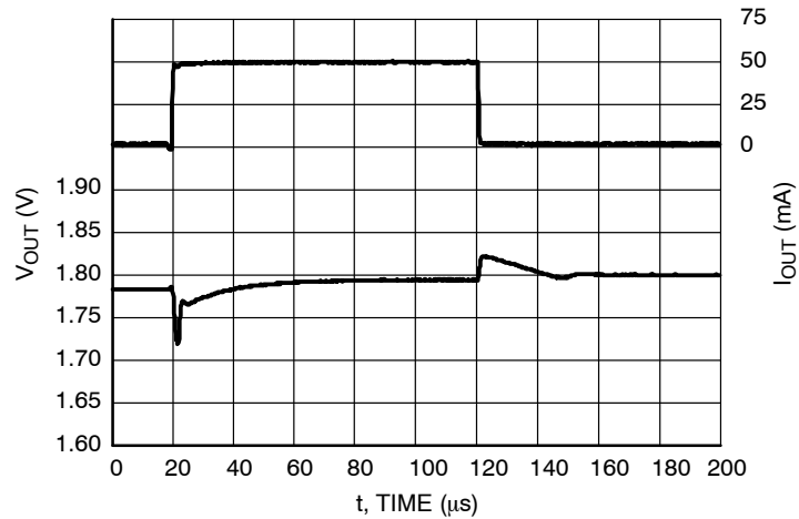
Figure 55. Load Transients, 1.8 V Version, I_{OUT} = 1 - 50 \text{ mA} , t_R = t_F = 0.5 \text{ } \mu\text{s} , V_{IN} = 2.8 \text{ V} , AE = 0 \text{ V}
