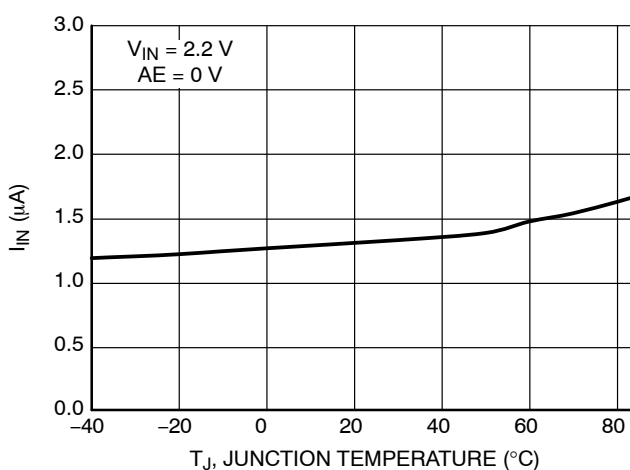
Figure 28. Supply Current vs. Temperature, 1.2 V Version
