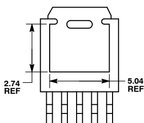
BOTTOM VIEW ALTERNATE CONSTRUCTION
