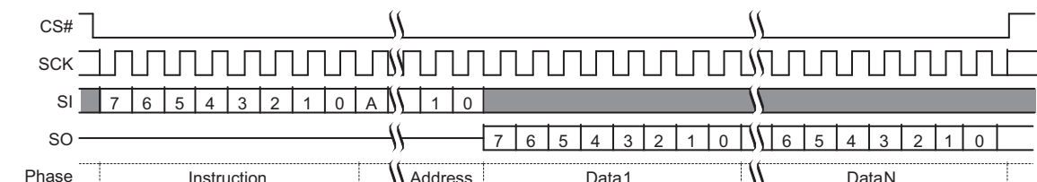
Figure 10.27 Read Command Sequence (3-Byte Address, 03h or 13h)
