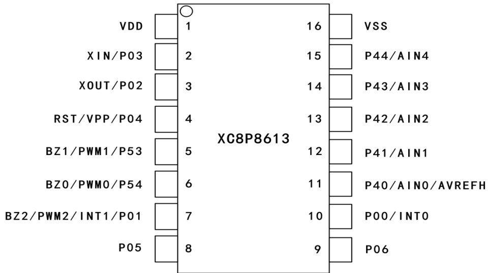
XC8P8613-16PIN 脚位图
