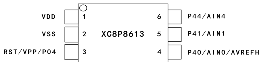
XC8P8613-6PIN 脚位图
