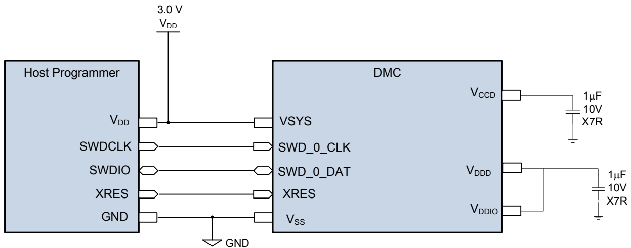
Figure 3. Connecting the Programmer to DMC Device
