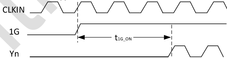
T_{1G\_ON} Output Enable Time
