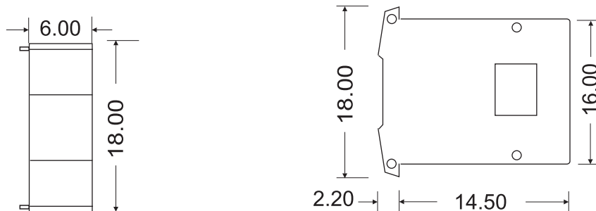
KA-3 SNAP-IN THE MOUNTING PLATE
