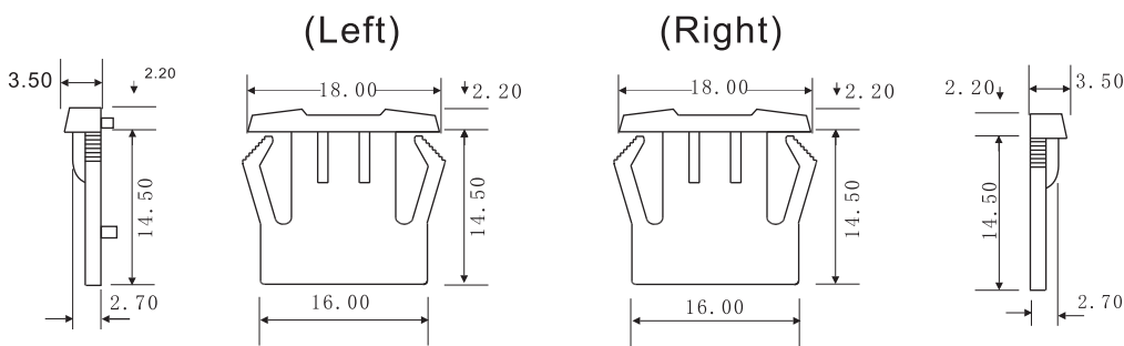
KA-3/03 SNAP-IN THE MOUNTING PLATE
