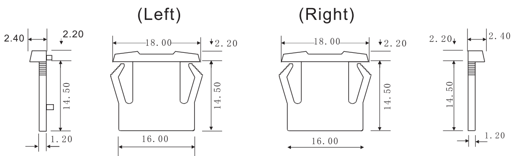
KA-3/03 SNAP-IN THE MOUNTING PLATE
