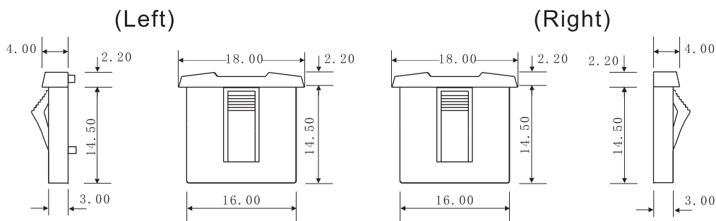
KA-3/02 SNAP-IN THE MOUNTING PLATE
