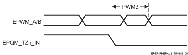
图 7-59. EPWM_A/B and ePWM_TZn_IN Forced High/Low Input Timings
