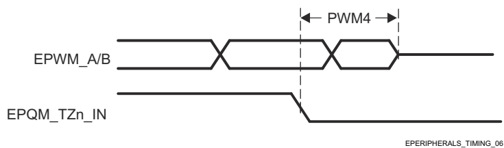
图 7-60. EPWM_A/B and ePWM_TZn_IN Hi - Z Input Timings
