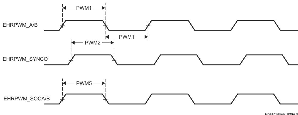
图 7-58. EPWM_A/B_out, ePWM_SYNCO, and ePWM_SOC/A/B Input Timings
