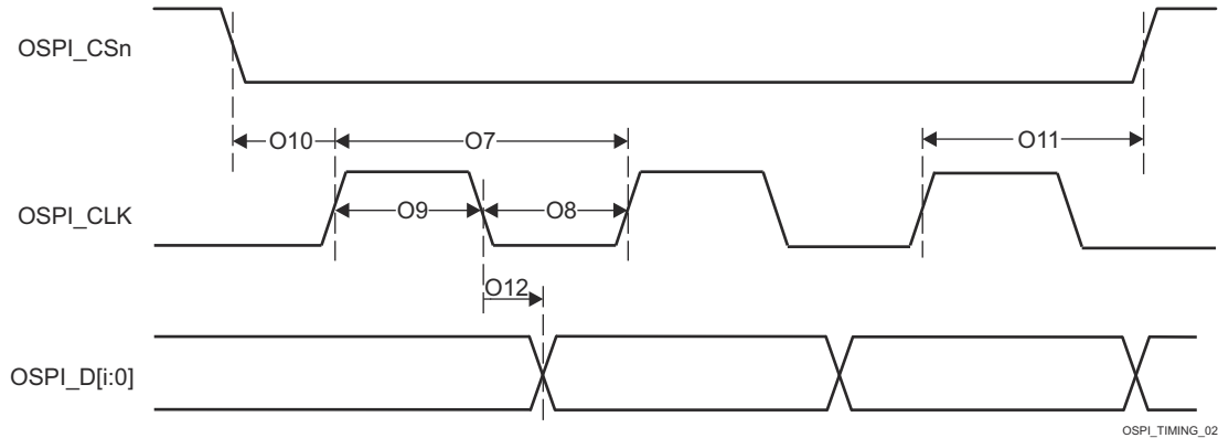
图 7-112. OSPI Switching Characteristics - SDR
