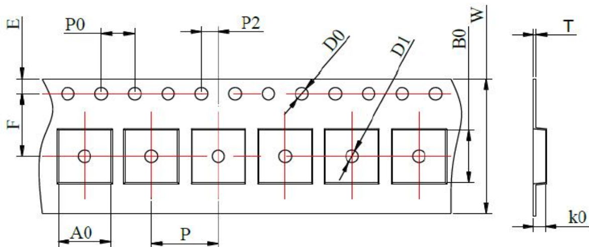
Tape dimensions (mm)
