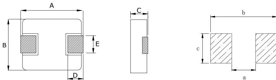
Recommend Land Pattern
