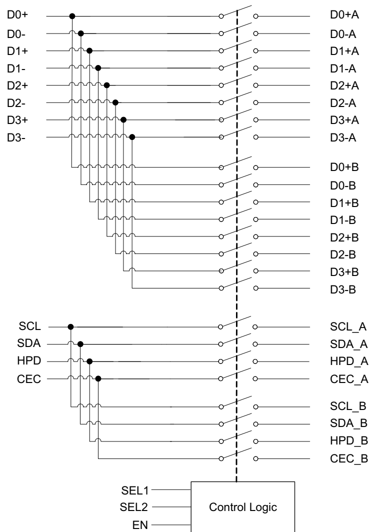
Figure 20. Logic Diagram
