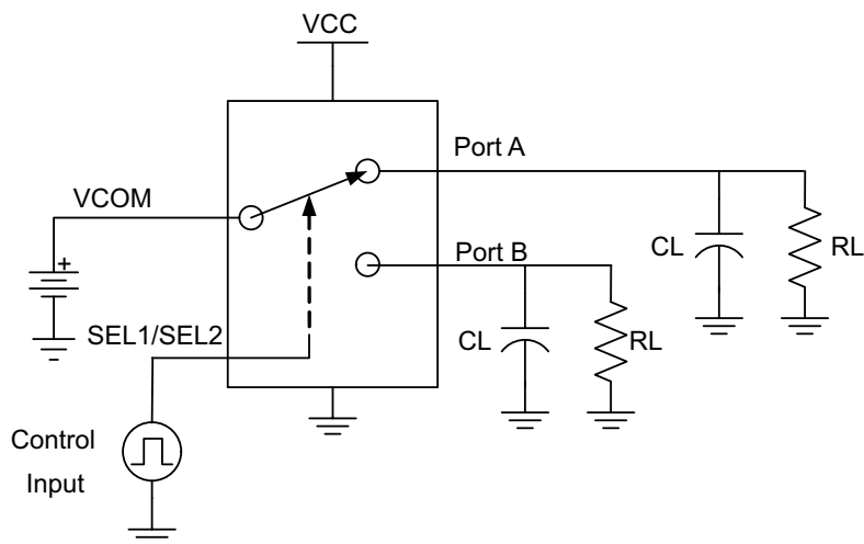
Figure 15. Switching Time Between Channels ( t_{\text{SWITCH}} )
