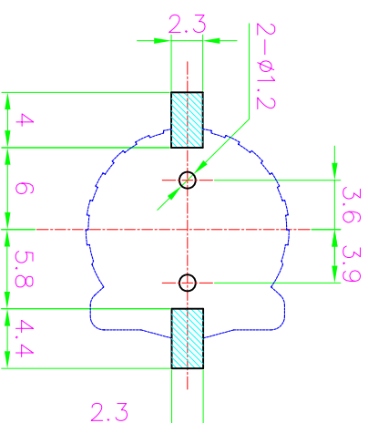
PCB Holes Diagram
