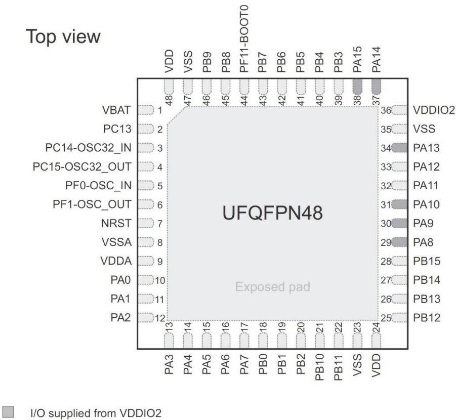
FCM32x042 UFQFPN48 pinout
