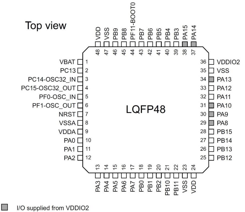
FCM32x042 LQFP48 pinout
