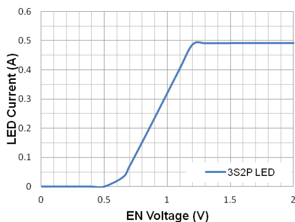
Figure 19. LED Current vs. EN Voltage ( V_{IN}=12V )
