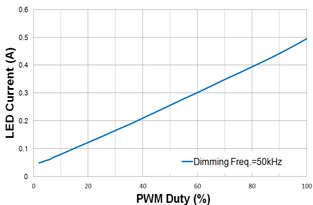
Figure 21. LED Current vs. PWM Duty ( V_{IN}=12V , 3S2P LED)
