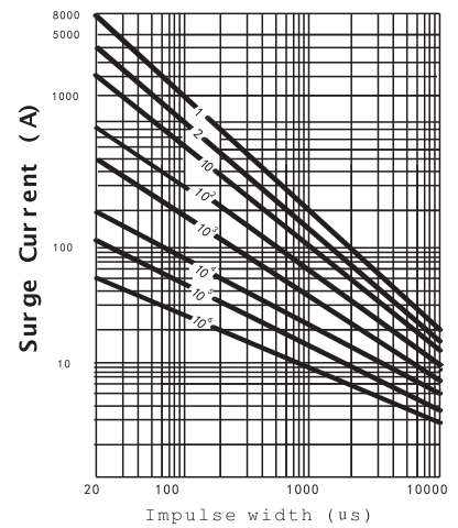
Impluse Lifetime Ratings FNR-40K180 to FNR-40K680
