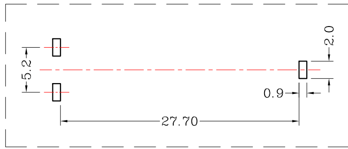
P.C.B MOUNTING
