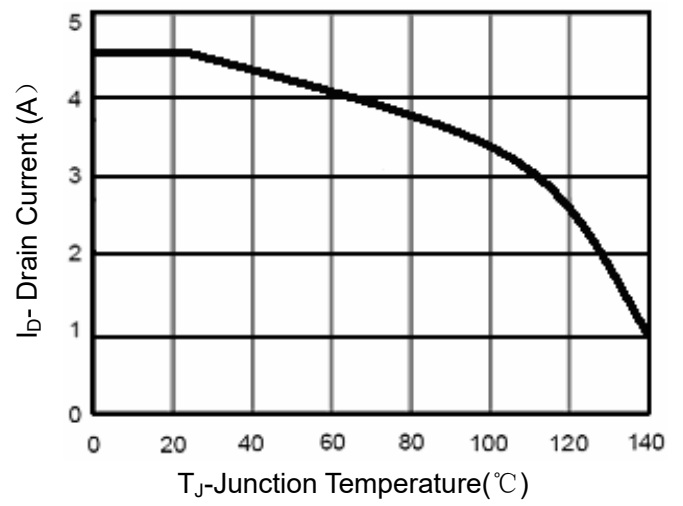
Figure 4 Drain Current
