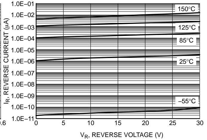
Figure 2. Reverse Leakage
