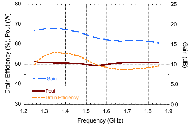
Gain & Drain Efficiency vs. Frequency ( P_{OUT} = 50 W)
