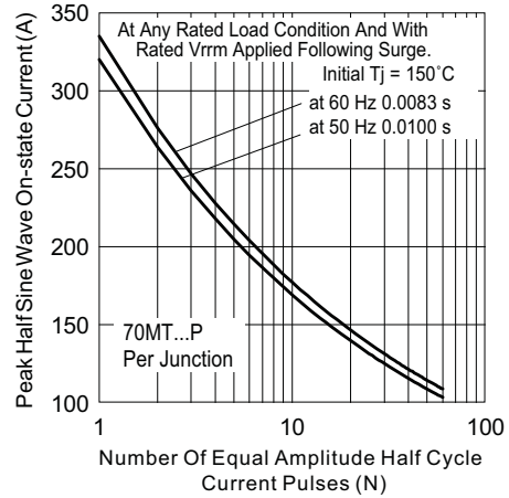
Fig. 8 - Maximum Non-Repetitive Surge Current
