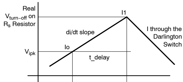
Figure 13. Current Waveform
