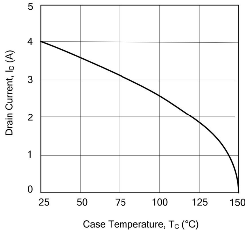
6. Maximum Drain Current vs. Case Temperature
