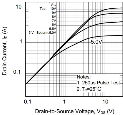
3. On-State Characteristics
