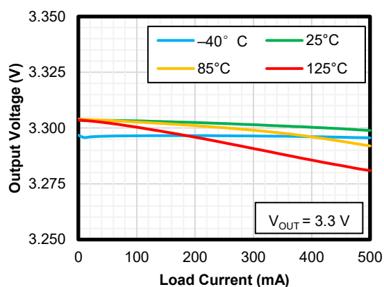
Figure 4 Load Regulation
