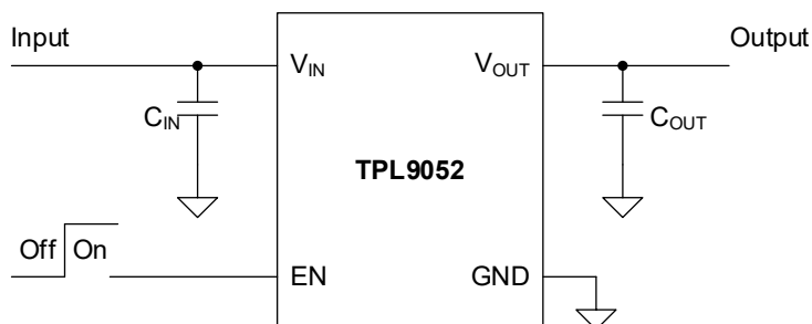
Figure 14 TPL9052 Typical Application Circuit
