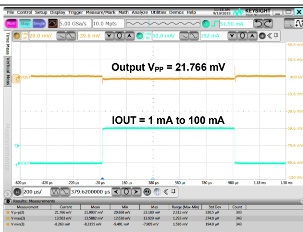
Figure 11 Load Transient
