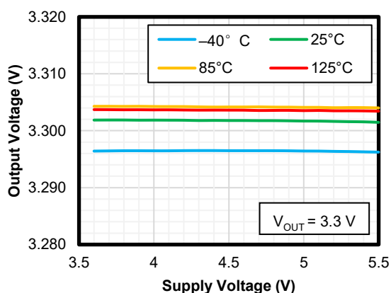
Figure 3 Line Regulation
