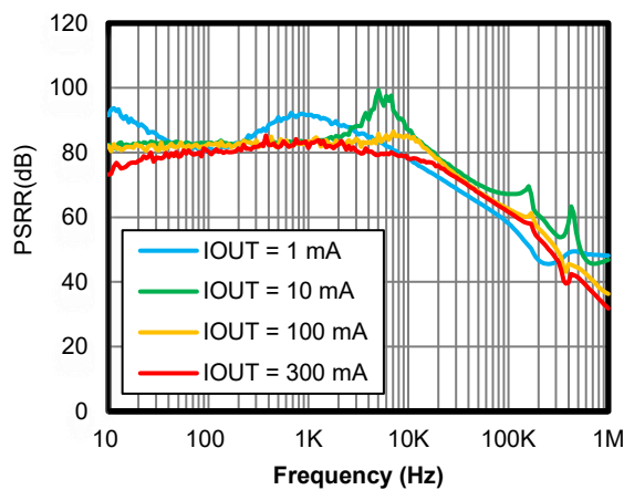
Figure 9 PSRR
