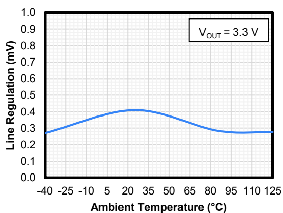
Figure 5 Line Regulation vs. Temperature
