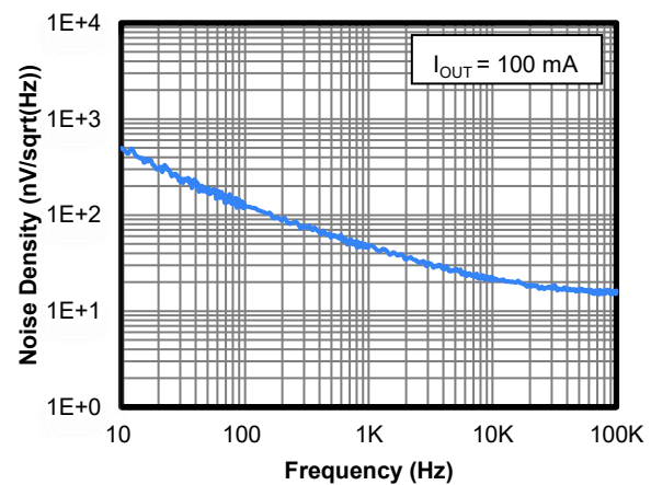
Figure 10 Noise
