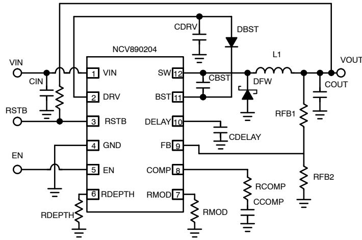
Figure 1. Typical Application
