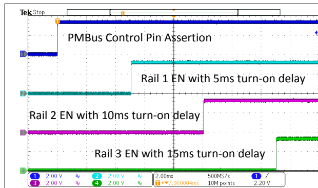
Figure 8-2. Example Power-On Sequence
