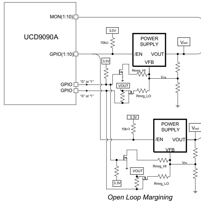
Figure 7-21. Open-Loop Margining
