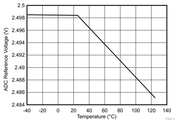
Figure 6-3. ADC Reference Voltage vs Temperature
