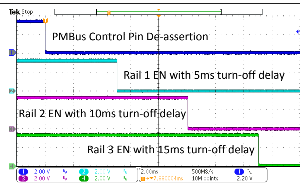
Figure 8-3. Example Power-Off Sequence
