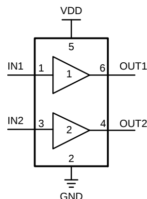
Figure 1. Simplified Logic Diagram
