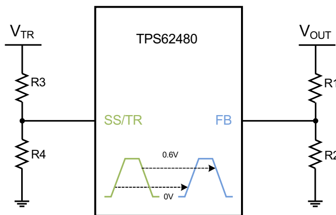
Figure 8. Voltage Tracking
