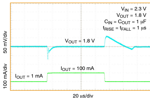
Figure 10. Load Transient Response, 1 mA – 100 mA NCV8752A/B, V_{OUT} = 1.8\text{ V}
