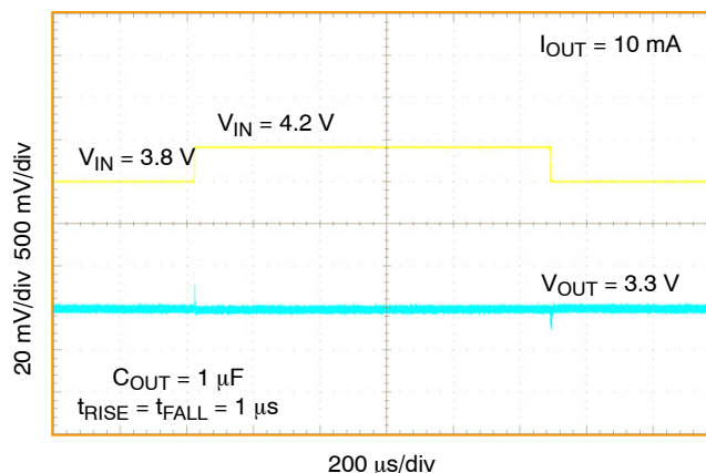
Figure 55. Line Transient 3.8 V – 4.2 V NCV8752A/B, V_{OUT} = 3.3\text{ V}
