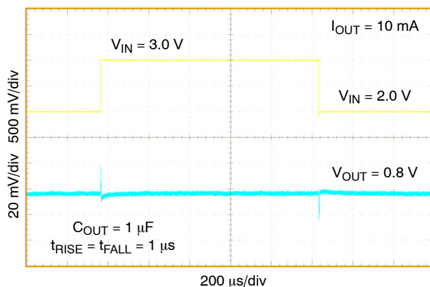
Figure 52. Line Transient 2 V – 3 V NCV8752A/B, V_{OUT} = 0.8\text{ V}
