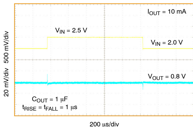
Figure 51. Line Transient 2 V – 2.5 V NCV8752A/B, V_{OUT} = 0.8\text{ V}
