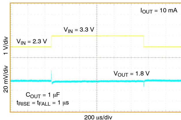
Figure 54. Line Transient 2.3 V – 3.3 V NCV8752A/B, V_{OUT} = 1.8\text{ V}
