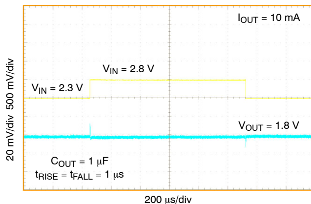
Figure 53. Line Transient 2.3 V – 2.8 V NCV8752A/B, V_{OUT} = 1.8\text{ V}
