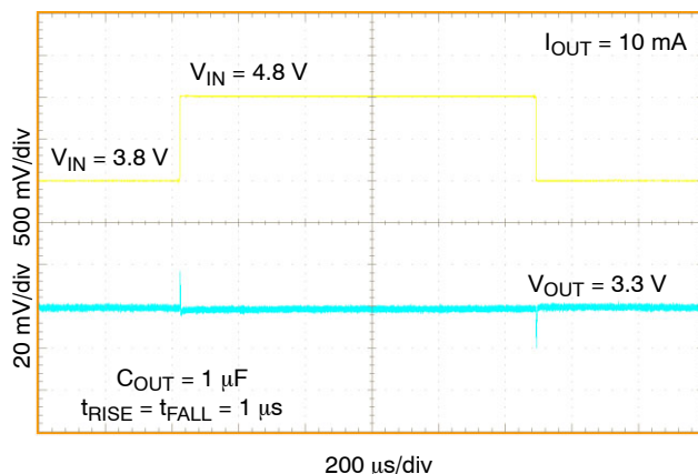
Figure 56. Line Transient 3.8 V – 4.8 V NCV8752A/B, V_{OUT} = 3.3\text{ V}
