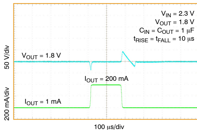
Figure 14. Load Transient Response, 1 mA – 200 mA NCV8752A/B, V_{OUT} = 1.8\text{ V}
