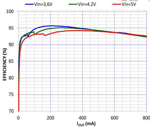
Figure 26. Efficiency vs Output Current vs PV_{IN} @25°C, F_{sw} = 3.429\text{ MHz} , V_{OUT} = 3.3\text{ V}
