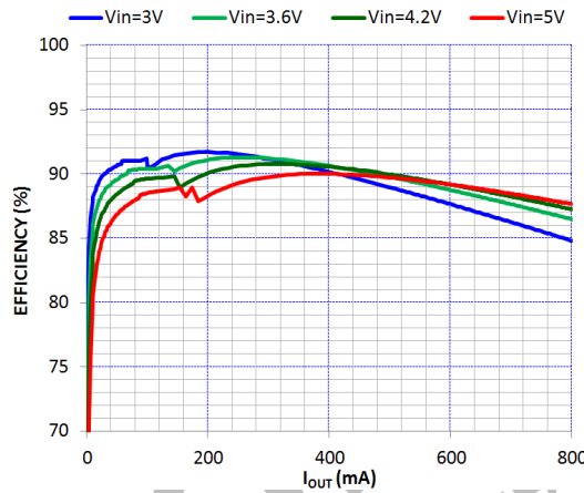
Figure 24. Efficiency vs Output Current vs PV_{IN} @25°C, F_{sw} = 3.429\text{ MHz} , V_{OUT} = 1.8\text{ V}
