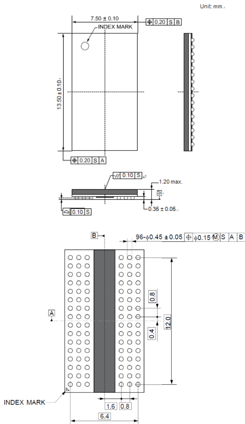
Figure 5 - Package outline(96ball FBGA)
