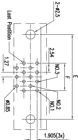
PCB Layout (14,26,50 Pos)
