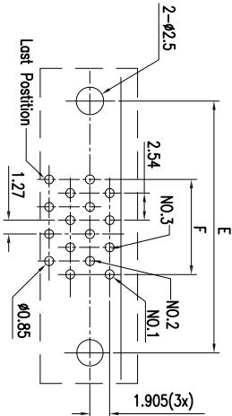
PCB Layout (20,36,40,68,100 Pos)
