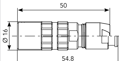
In Line Cable (PC)*
