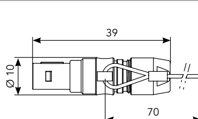
Straight Plug with Lanyard (FN)*
