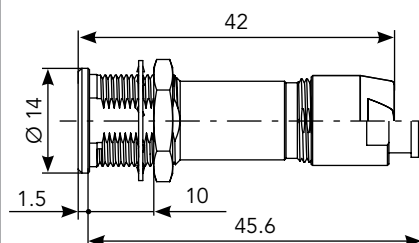
Front Mount Cable (SR)*
