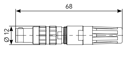
Straight Plug (FF)
