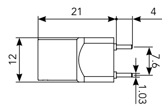
PCB Rear Mount with Mounting Pins (EZ)
