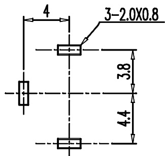
P.C.B HOLE LAYOUT BOTTOM VIEW
