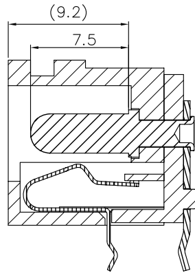
SECTION A-A (插针规格: Ø3.0)
