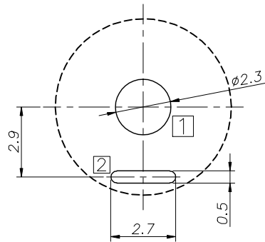
RECOMMENDED P. C. B. LAYOUT UNSPECIFIED TOLERANCE: ±0.05 (TOP VIEW)
