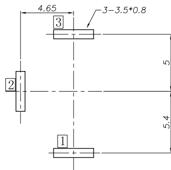
Recommended PCB Layout (Tolerance \pm 0.05 ) (Copper-sided View)
