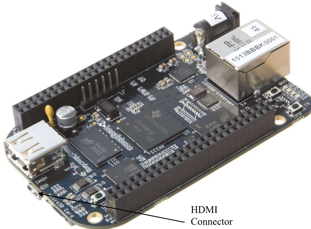
Figure 57. HDMI Connector
