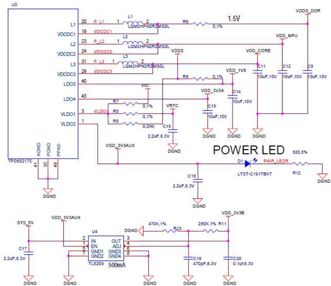
Figure 25. Power Rails
