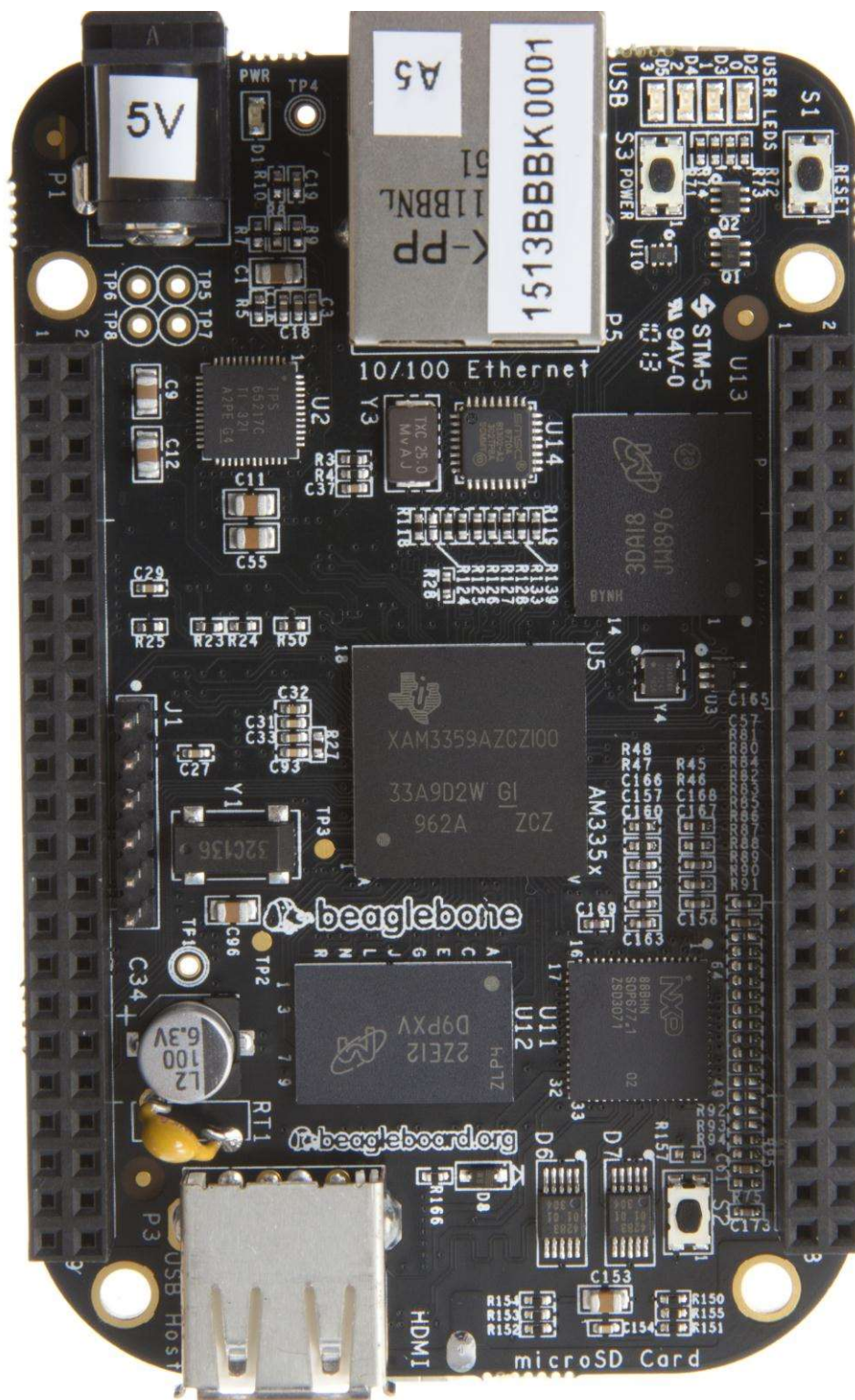
Figure 74. Top Side
