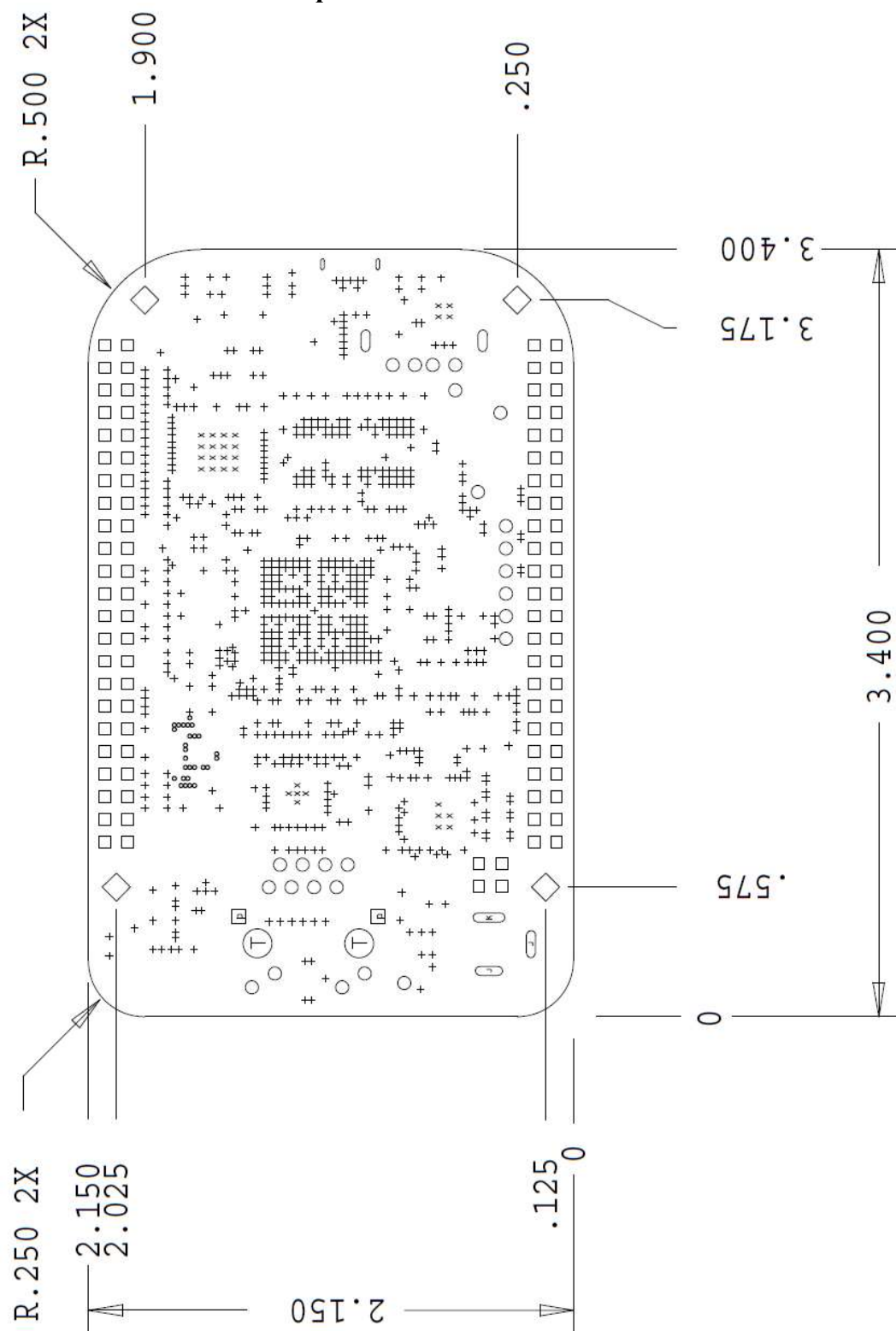
Figure 71. Board Dimensions
