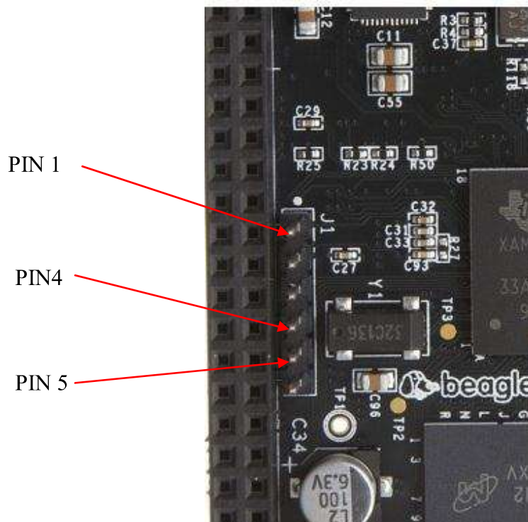
Figure 56. Serial Header
