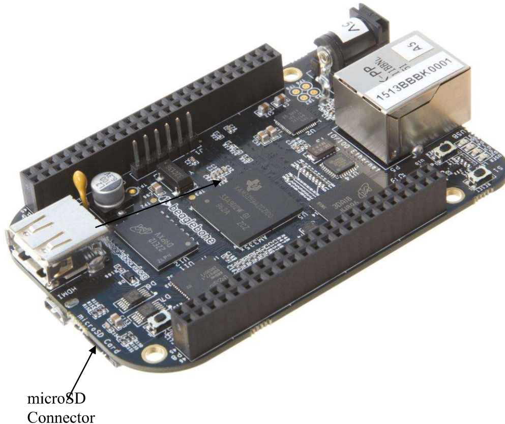
Figure 59. microSD Connector
