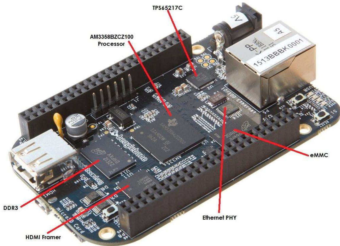
Figure 18. Key Components
