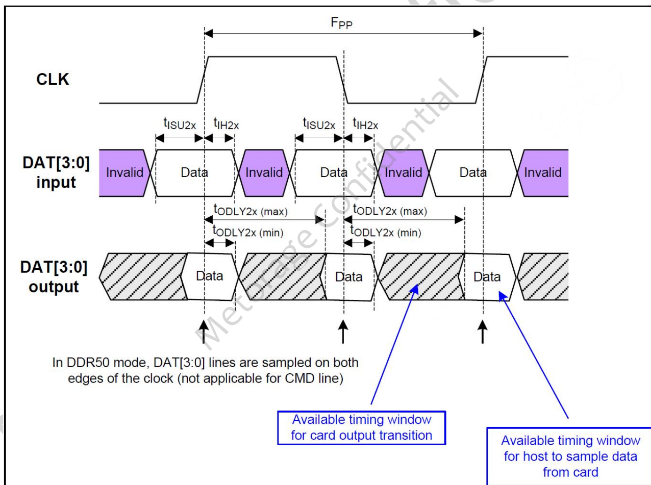
Figure 5-11 Timing Diagram DAT Inputs/Outputs Referenced to CLK in DDR50 Mode
