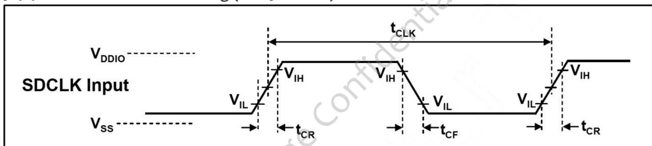
Figure 5-10 Clock Signal Timing
