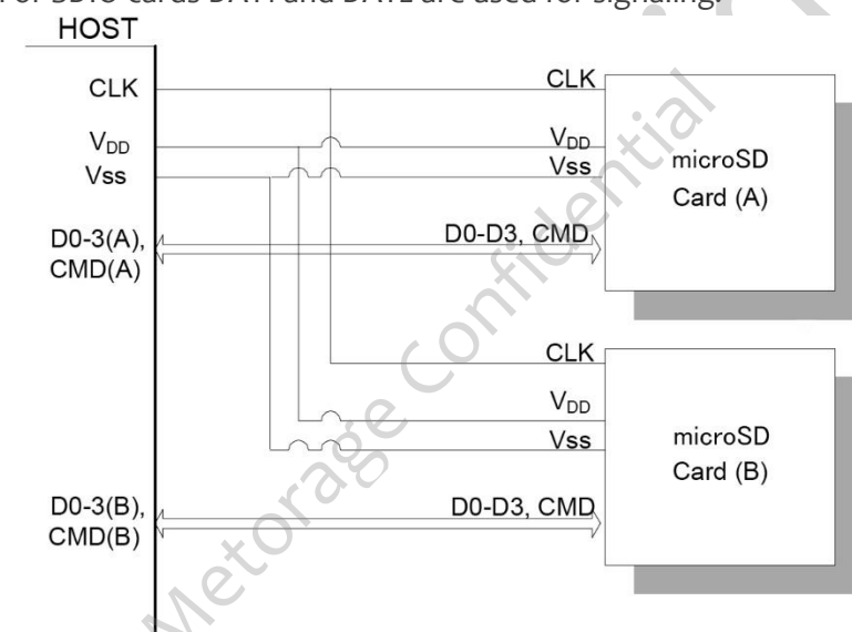
Figure 3-2 SD Memory Card System Bus Topology
